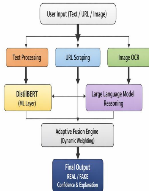
Fig. 1. Proposed multi-layer hybrid fake news detection architecture integrating ML, LLM, and adaptive fusion.
