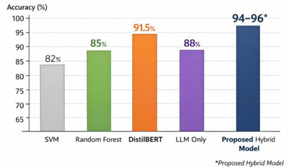
Fig. 2. Accuracy comparison across baseline models and proposed hybrid system.
